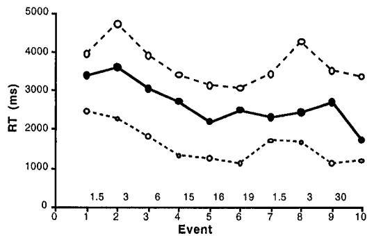
Fig. 5. Bracketing models for the Keypad Interface. Predicted RTs are shown as open points; observed as solid.
