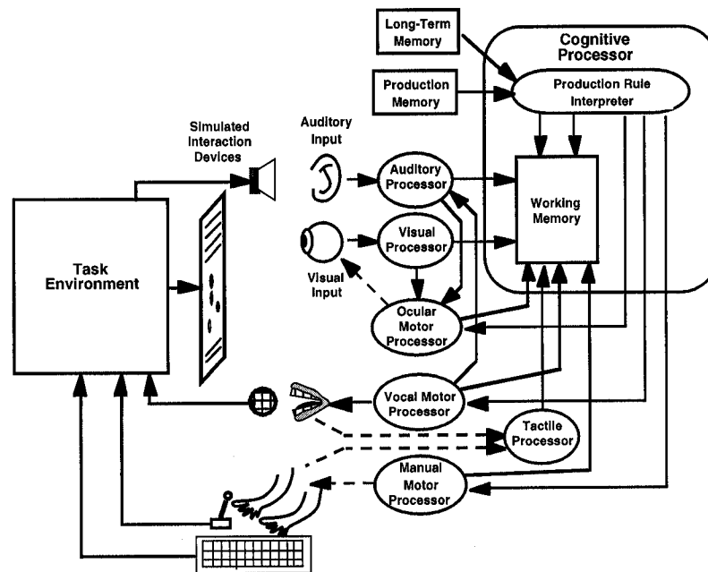
Fig. 3. The overall structure of the EPIC architecture. Perceptual-motor peripherals surround a cognitive processor.
