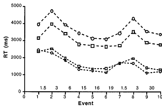
Fig. 7. Predicted RTs for fastest-possible (small points) and slowest-reasonable (large points) models for the Keypad (circles) and Touchscreen (squares) interfaces.
