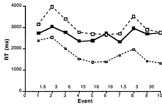
Fig. 6. Bracketing models for the Touchscreen Interface. Predicted RTs are shown as open points; observed as solid.
