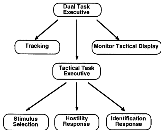
Fig. HIERARCHY. The structure of the production-rule task strategy for both interfaces.
